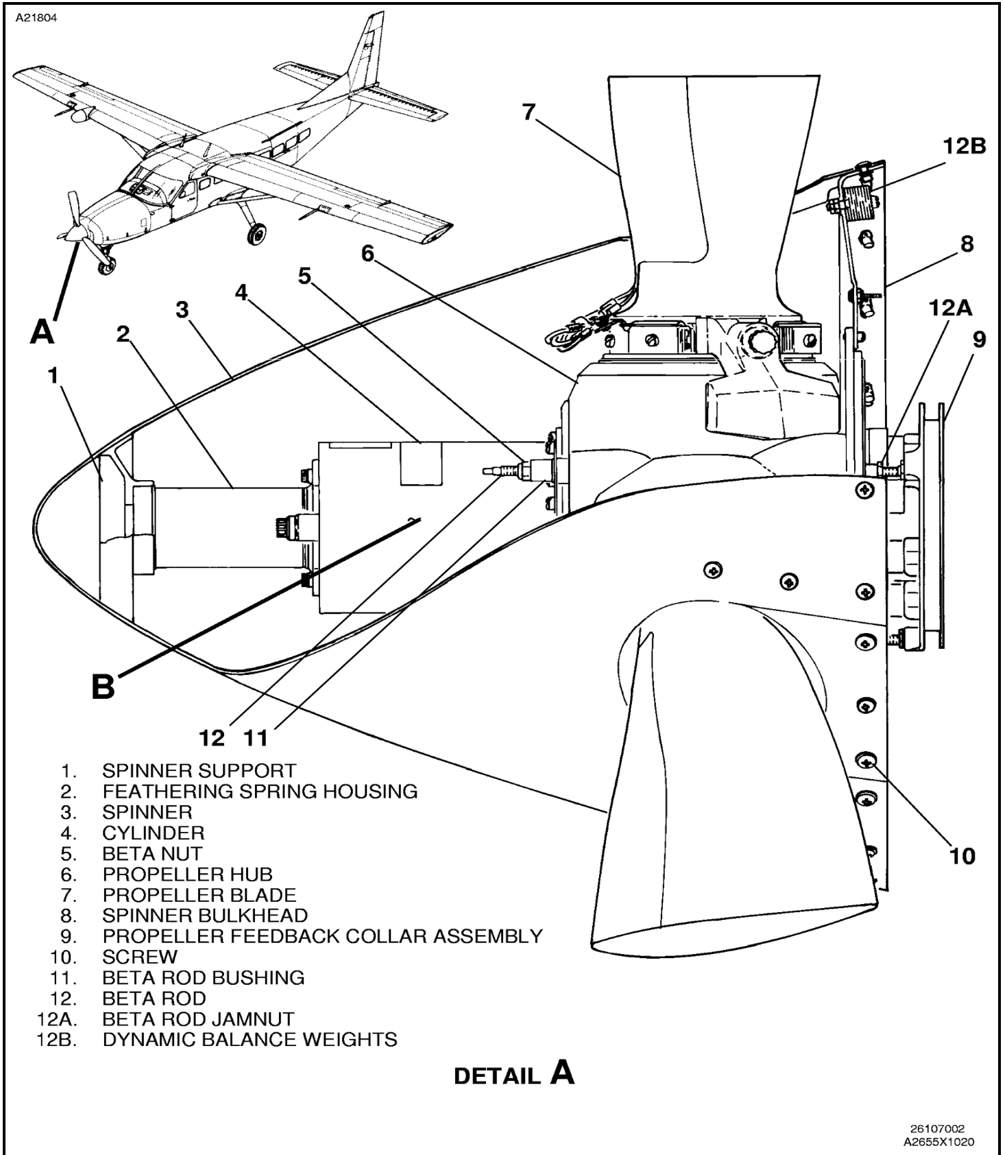
Figure 1 : Sheet 1 : McCauley Propeller Assembly Cutaway
